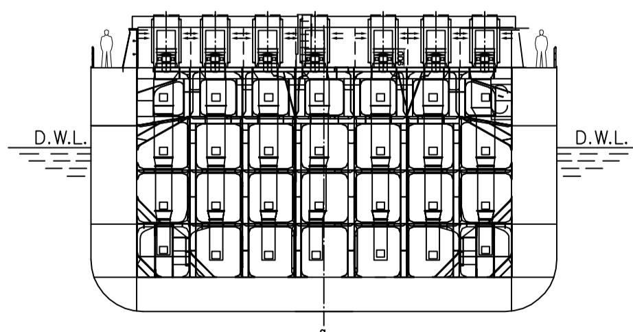
FRAME 60,5 and 103,5 MECHANICAL SUPPLY
