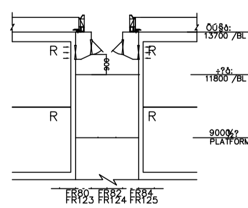
FRAME 80 and 123 NATURAL EXHAUST
